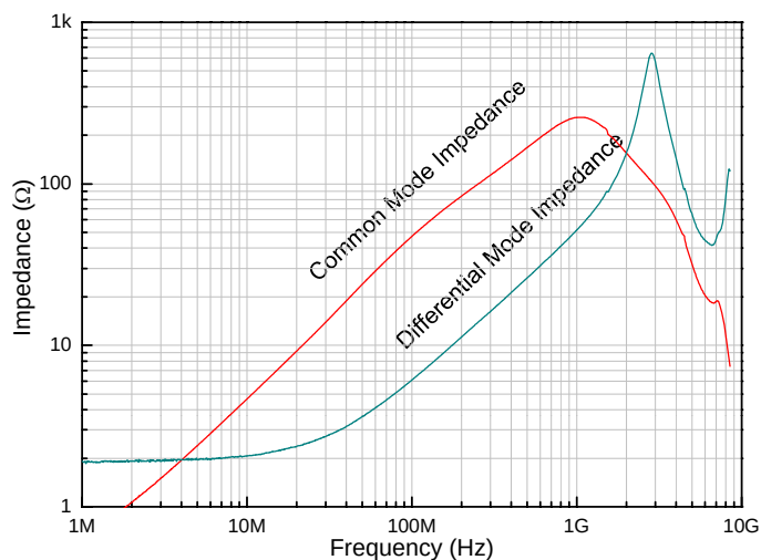
- Impedance Curves
