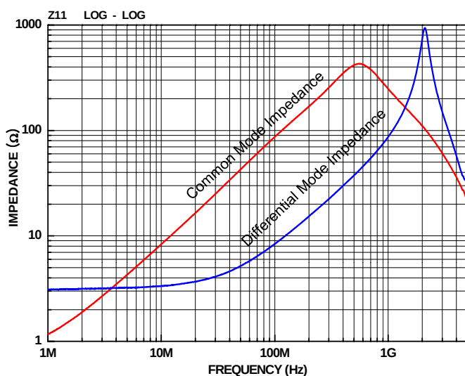
- Impedance Curves
