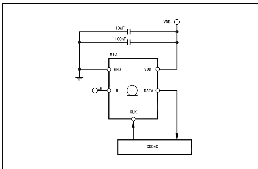
Figure 1. MSM261D4030Z1CM electrical connections
