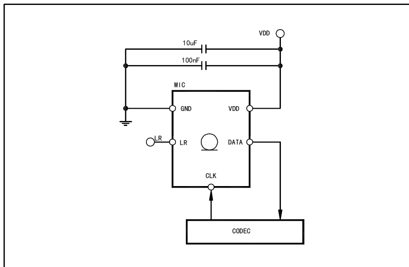
Figure 1. MSM261DCB001 electrical connections
